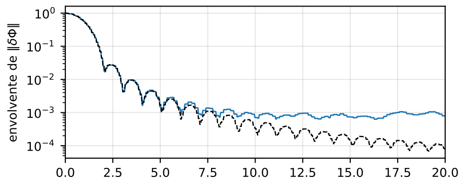
D2: \eta = 0.6 , en la banda, lineal ( \nu = 0.3 )
