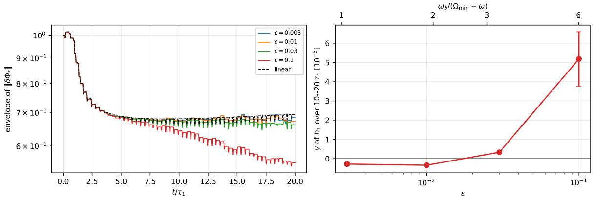
Figure 6: The \varepsilon scan of the mode of L5. Left: envelopes of \|\delta\Phi_\varepsilon\| at four amplitudes and linear theory. Right: \gamma of h_1 over 10 – 20\tau_1 as a function of \varepsilon , with the ratio \omega_b/(\Omega_{\min} - \omega) on the top axis.
