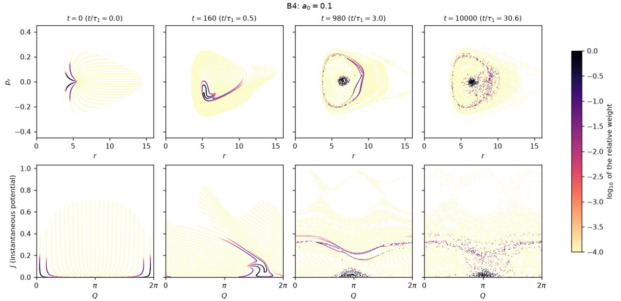
Figure 25: B4: the blob with a_0 = 0.1 . It collapses in the first radial periods into a dense core ( r \approx 6.5 , p_r \approx 0 at these times) with 79 % of the mass, surrounded by a halo of stripped particles. In (Q, J) the core is at J \approx 0 : it is the nearly circular orbit of the potential that it creates.
