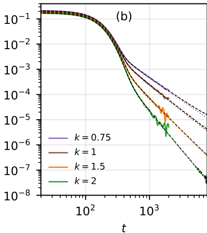
polytropes, M_{gas}/M = 0.01
