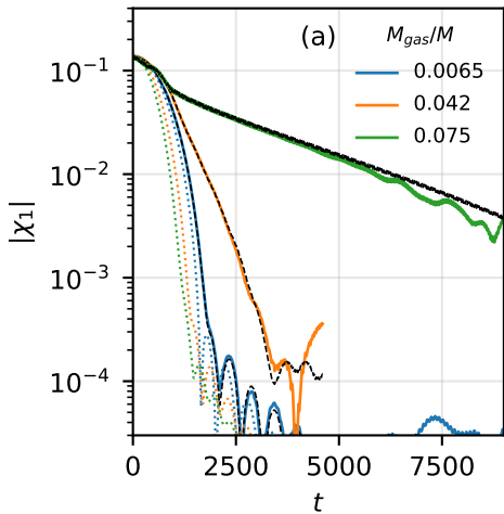
lowered Maxwellians, g = 2
