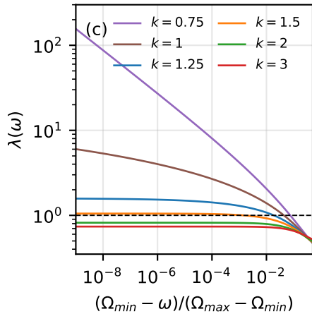
polytropes, M_{\text{gas}}/M = 1
