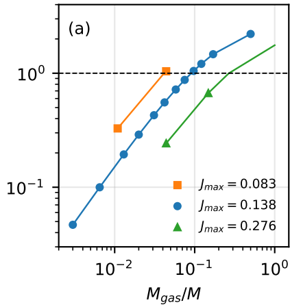
lowered Maxwellians, g = 2
