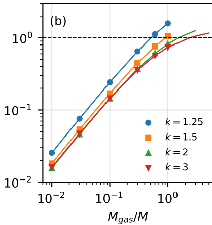
polytropes
