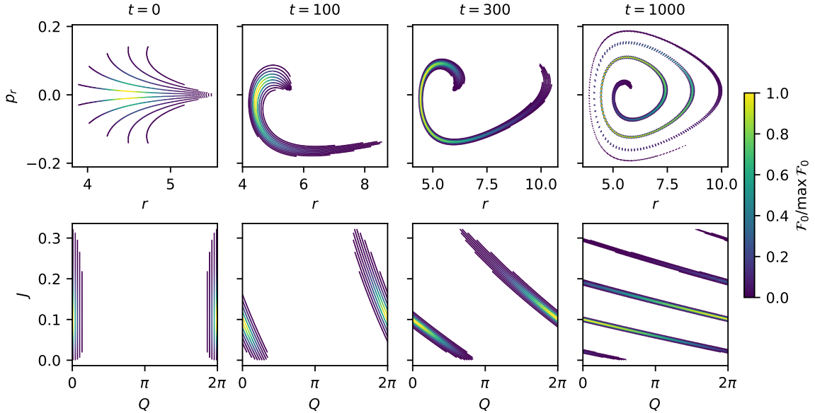
FIG. 1: Mixing of the initial datum (74) in the isochrone potential when self-gravity is neglected. Shown are the computational particles in the (r, p_r) -plane (upper panels) and in the plane of the action-angle variables (lower panels) at four different times, for a lattice with N_J \times N_Q = 800 \times 64 points. The color indicates the mass of each particle relative to the largest one, and only particles whose mass exceeds 10^{-3} of the latter are shown.
