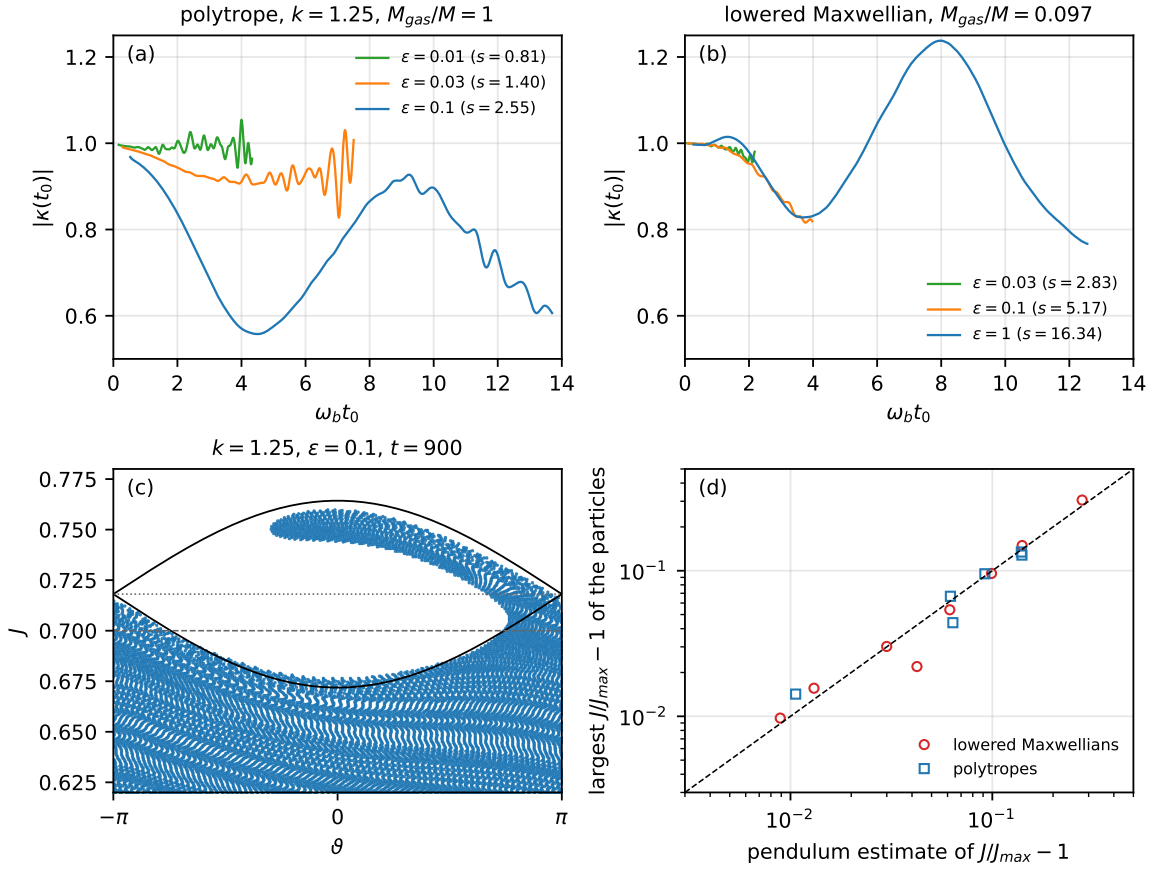
FIG. 9: Effect of the amplitude of the perturbation on the oscillating mode. (a) Ratio |\kappa(t_0)| between the amplitudes of the response obtained from the PIC code and from the linearized equations, see Eq. (81), as a function of time in units of the inverse bounce frequency, for the polytrope with k = 1.25 and M_{gas}/M = 1 and three amplitudes ( N = 1.024 \times 10^5 ). (b) The same for the lowered Maxwellian with g = 2 and M_{gas}/M = 0.097 ( N = 10^4 ). (c) The computational particles near the edge of the steady state for the simulation with \varepsilon = 0.1 of panel (a) at t = 900 , which corresponds to half a bounce period, in terms of the angle (87) and the action variable. The solid lines are the separatrix (91), the dashed line indicates J_{max} and the dotted one J_r . (d) Largest value of the action variable attained by the computational particles in the simulations of Table VIII, compared to the value J_+ predicted by the pendulum (90).
