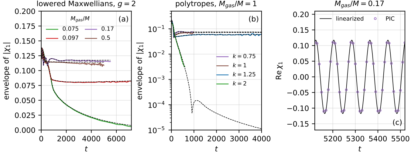
FIG. 8: Response of the gas for steady states above the threshold mass. (a) Envelope of |\chi_1(t)| (largest value in a moving window of width 100) for the lowered Maxwellians with g = 2 and J_{max} = 0.138 , obtained from the PIC simulations with \varepsilon = 0.075, 0.01, 0.1 and 0.1 in the order of increasing mass (solid lines) and from the linearized equations (dashed lines). The case M_{gas}/M = 0.075 , which lies below the threshold, is included for comparison. (b) The same for the polytropes with M_{gas}/M = 1 , with a window of width 50. The PIC simulations have \varepsilon = 0.1 and are shown for t \leq 1000 ( t \leq 600 for k = 2 ), except for k = 1.25 , where \varepsilon = 0.01 and N = 1.024 \times 10^5 . (c) Real part of \chi_1 at the end of the simulation for the lowered Maxwellian with M_{gas}/M = 0.17 .
