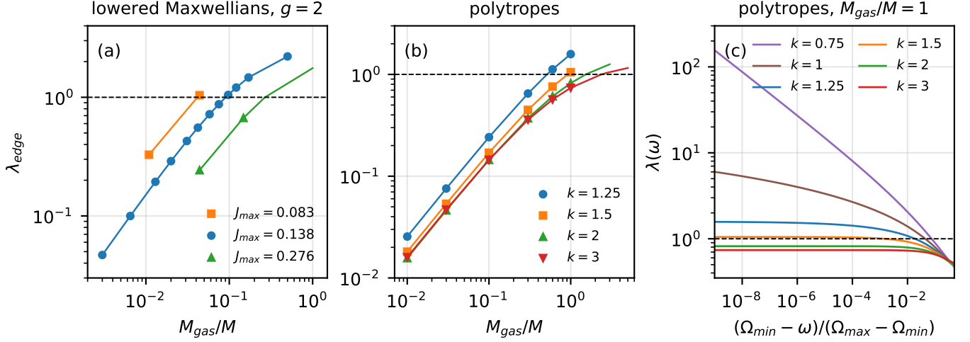
FIG. 6: Gain of the self-consistent loop. (a) The value \lambda_{edge} at the edge of the frequency band as a function of the mass of the gas, for the lowered Maxwellians with g = 2 in the isochrone potential and three values of J_{max} . (b) The same for the polytropes with k > 1 in the Kepler potential. The symbols refer to the steady states of section VI A, and the lines include those which were computed in order to determine the threshold mass. (c) The gain as a function of the distance (82) from the edge of the band, for the polytropes with M_{gas}/M = 1 . An oscillating mode exists if and only if the curve crosses the dashed line \lambda = 1 .
