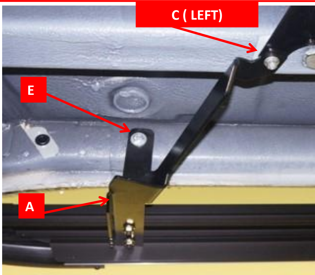
FRONT BRACKET
