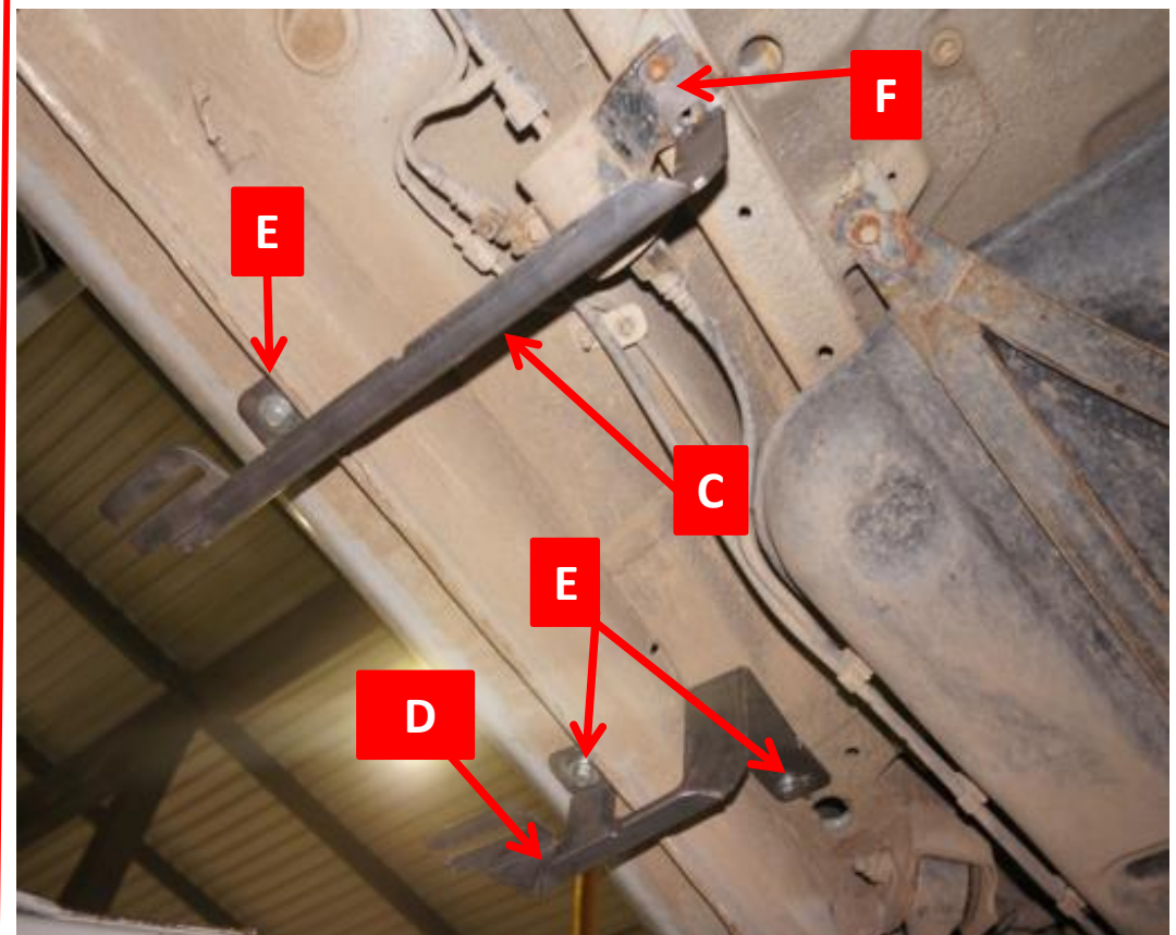
MIDDLE-REAR BRACKET
