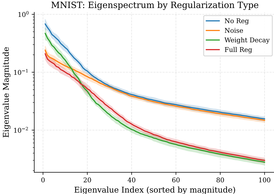
Figure 1: Eigenspectrum comparison across regularization configurations on MNIST. Weight decay (WD) produces the sharpest spectral decay with effective rank \sim 21 , while noise augmentation alone increases effective rank to \sim 75 . The combination (Full) achieves a moderate effective rank of \sim 36 . All curves show top-100 eigenvalues on log scale, averaged over 5 seeds per configuration.
