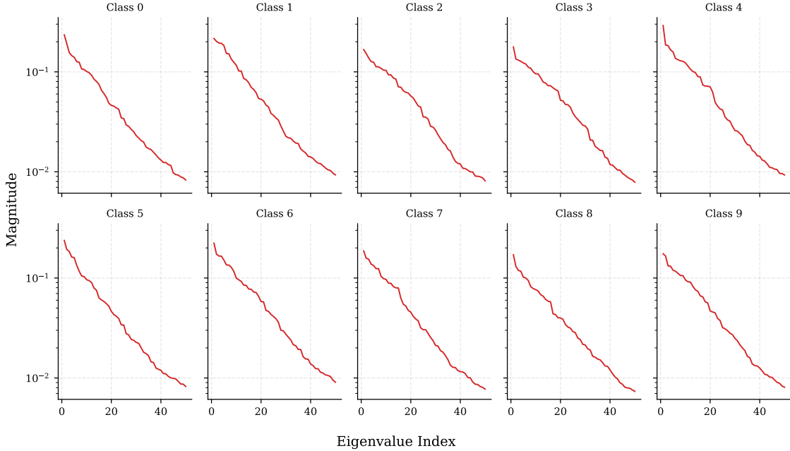
Figure 3: Per-class eigenspectrum for the fully regularized MNIST model. Each line represents a digit class (0–9). All classes show similar low-rank structure with approximately 10–15 significant eigenvalues, consistent with the paper’s claims about class-specific interpretability.
