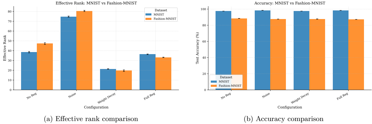
Figure 7: Cross-dataset comparison between MNIST and Fashion-MNIST. Both datasets show consistent trends: weight decay produces the lowest effective rank, while noise augmentation increases it. Fashion-MNIST has lower overall accuracy but similar relative patterns across configurations.
