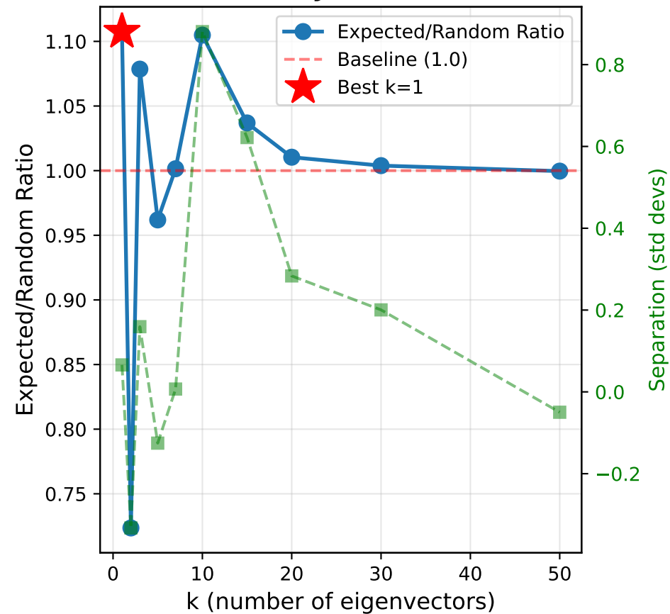
Projection
