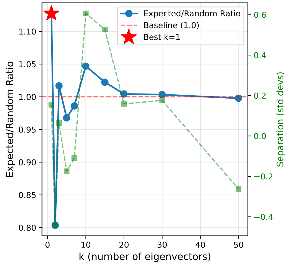
Grassmann
