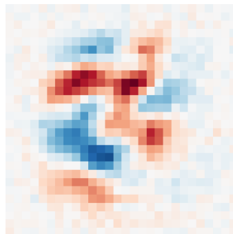
Class 3 (0.84)
