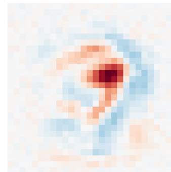
Class 9 (2.29)
