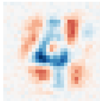
Class 4 (1.73)
