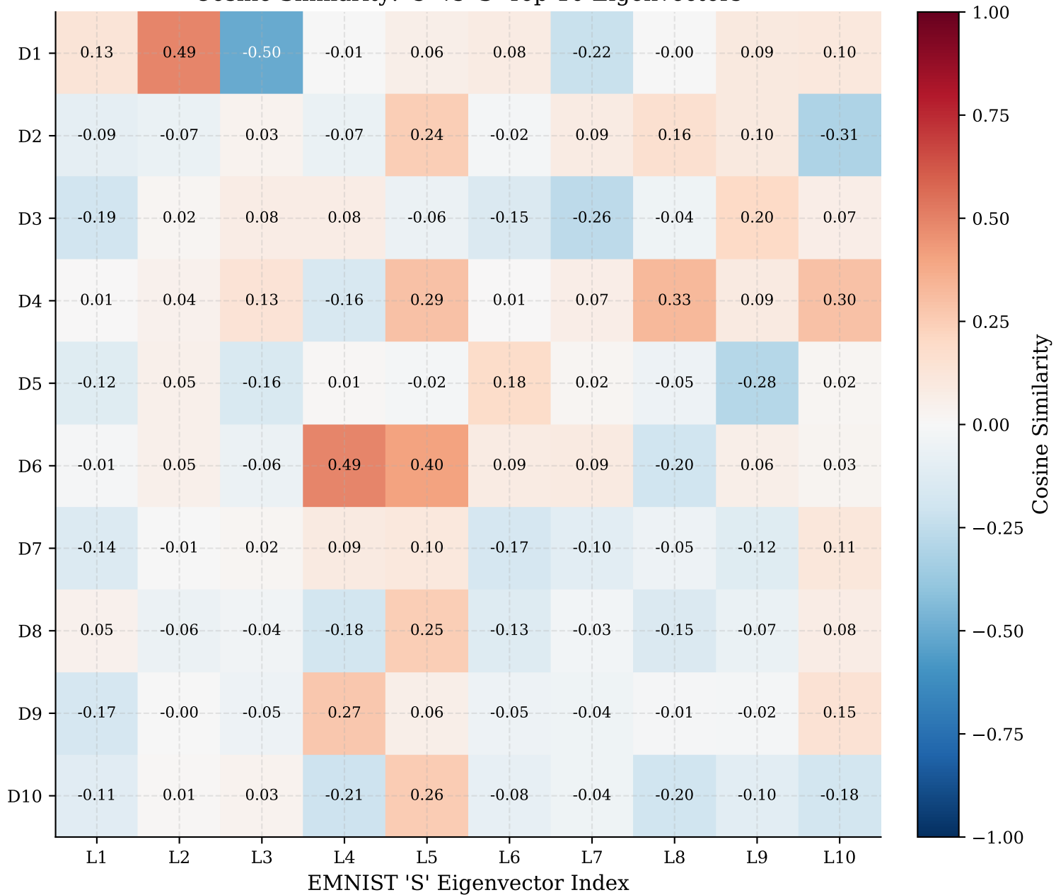
Cosine Similarity: '5' vs 'S' Top-10 Eigenvectors
