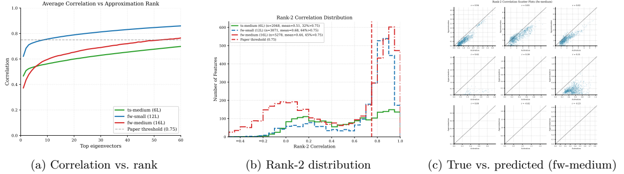
Figure 5: Low-rank correlation (Paper Figure 9). ts-medium (L4, \text{exp}=4 , n=2048 ), fw-small (L8, \text{exp}=4 , n=3072 ), fw-medium (L10, \text{exp}=8 , n=5688 ).
