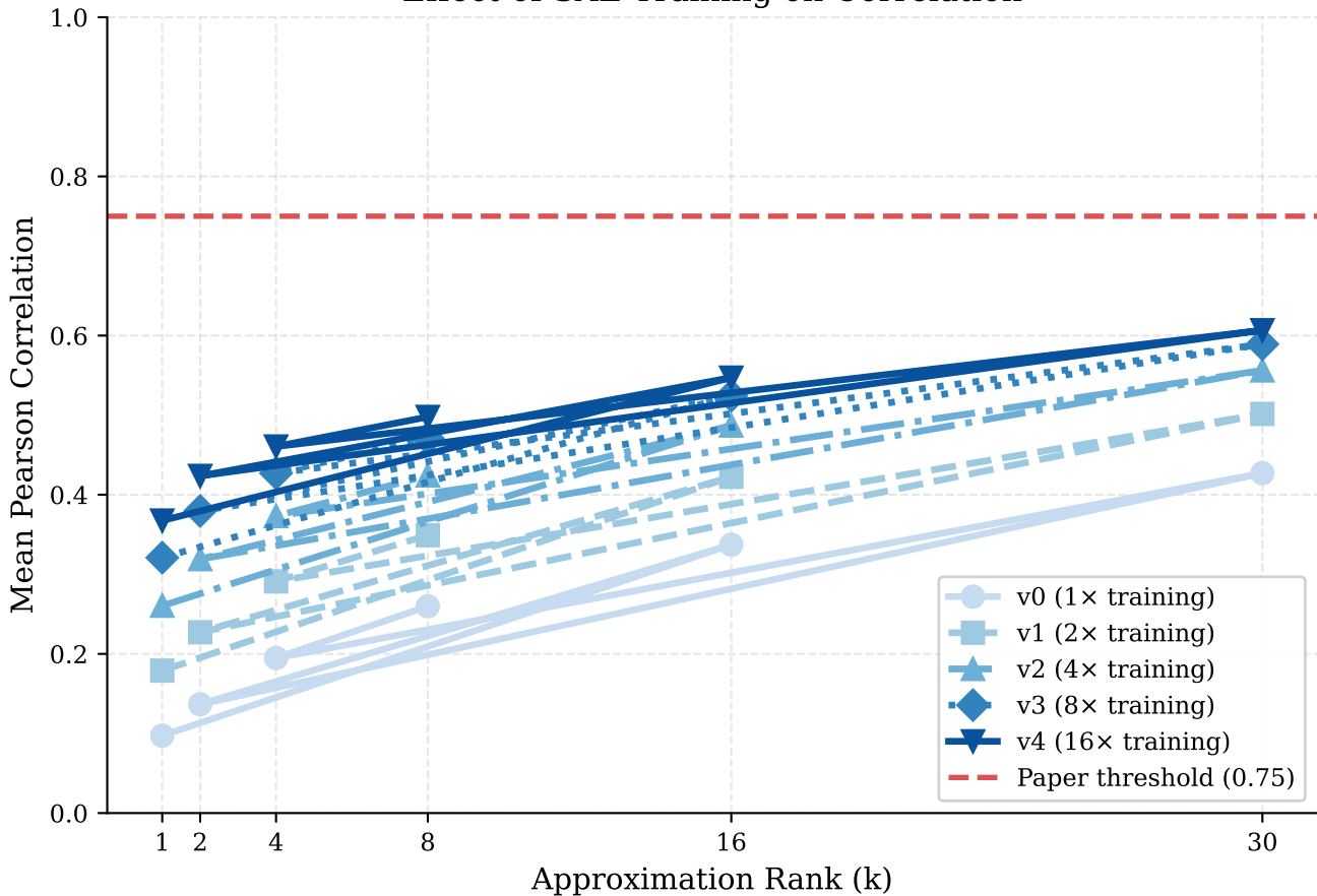
Effect of SAE Training on Correlation
