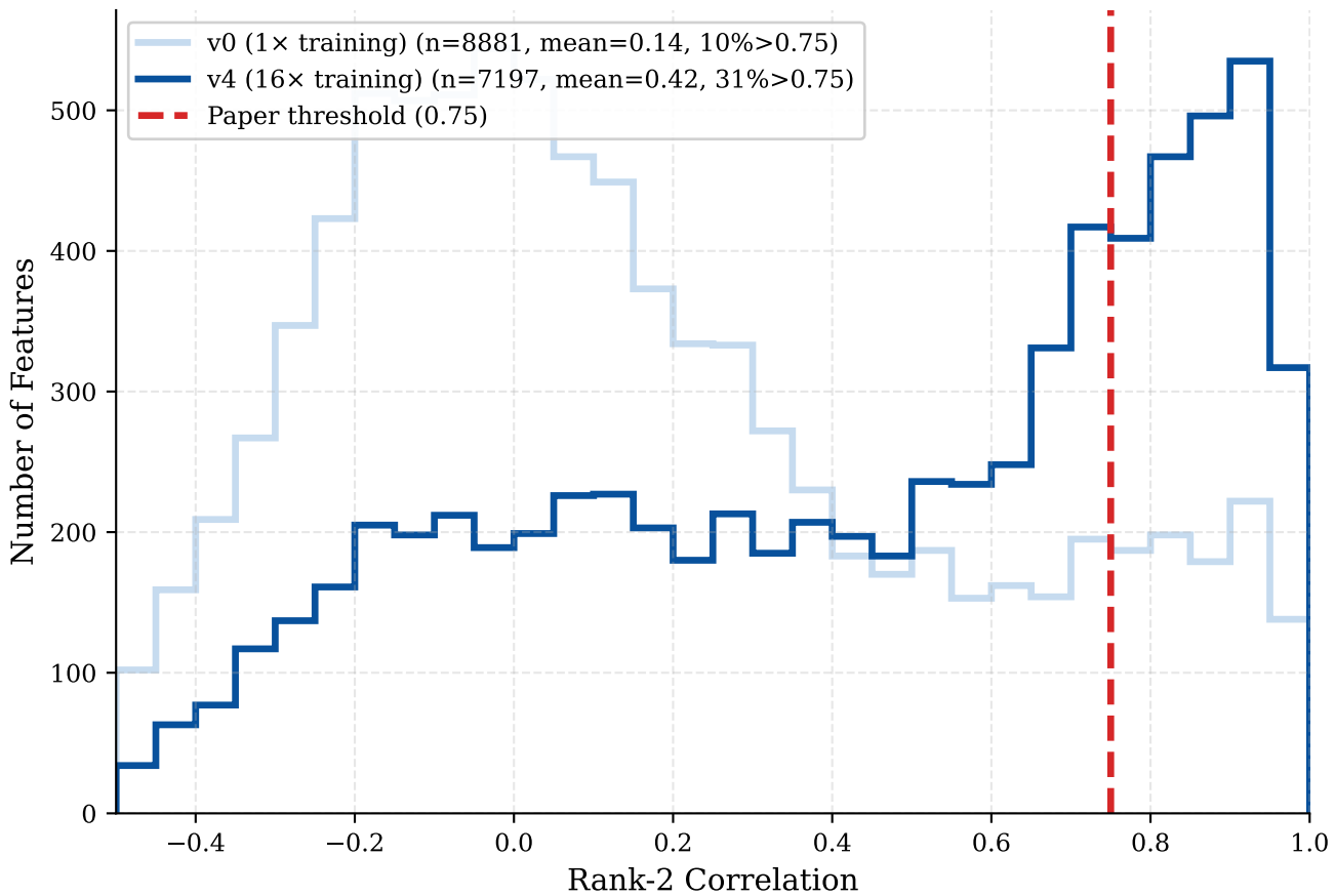
Rank-2 Correlation: v0 vs v4
