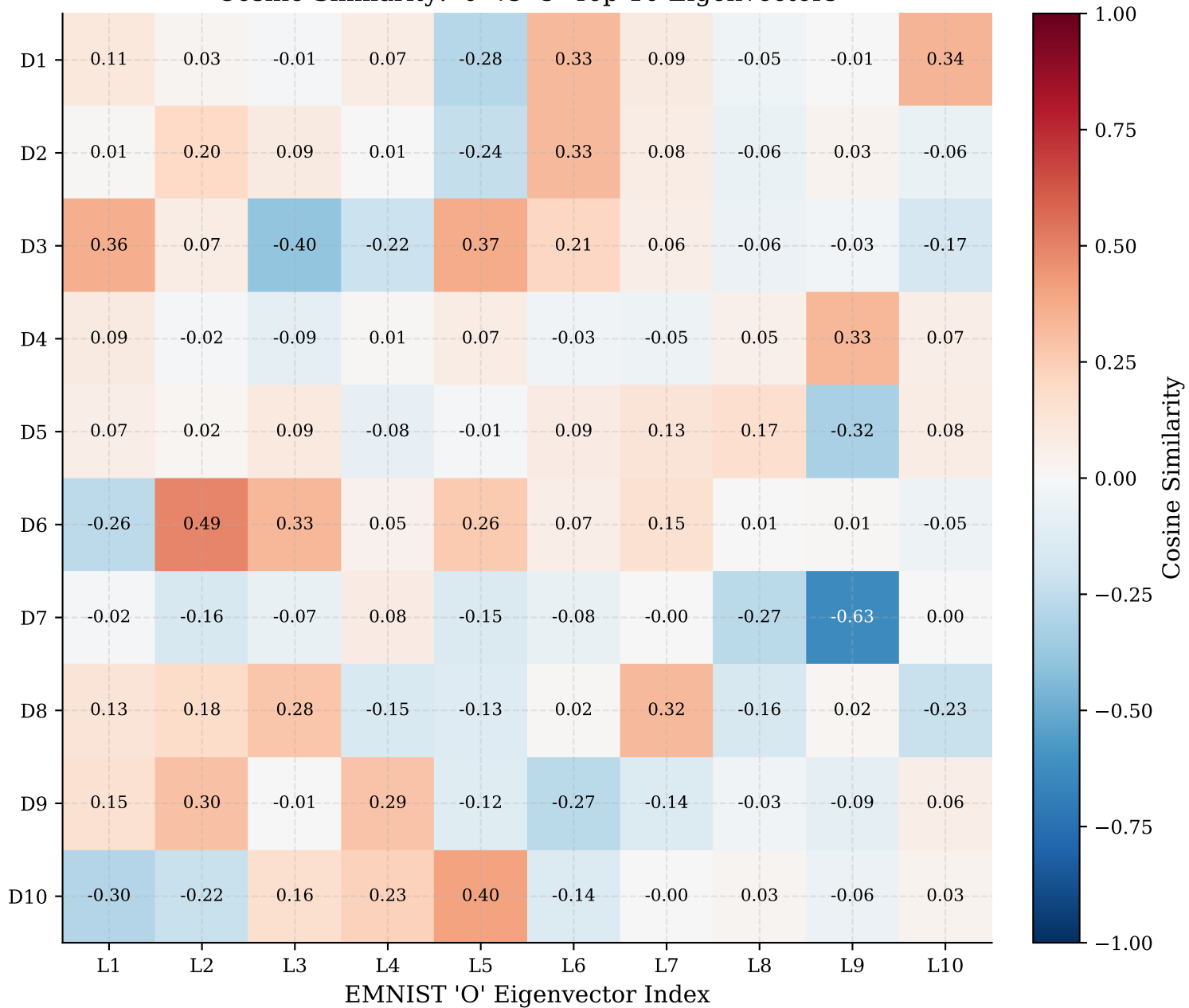
Cosine Similarity: '0' vs 'O' Top-10 Eigenvectors
