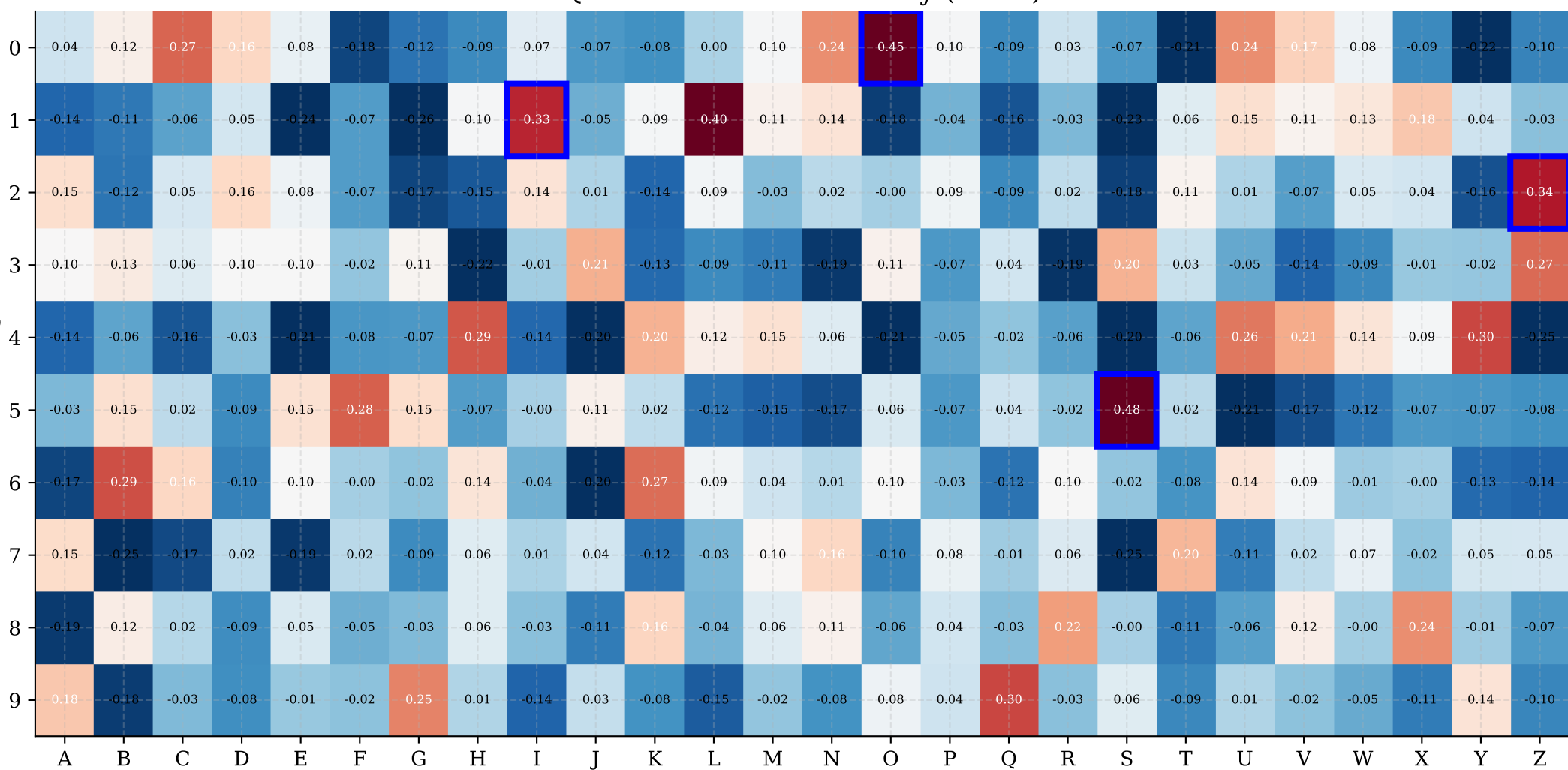
Quadratic Form Similarity (k=20)
