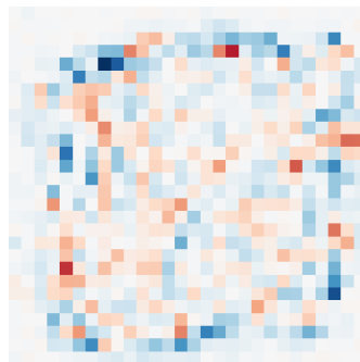
\lambda=-1.29
