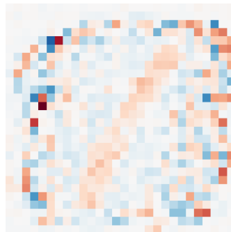
\lambda=0.90
