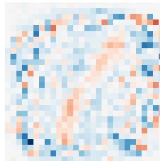
\lambda=0.50
