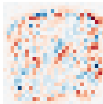
\lambda=-1.10
