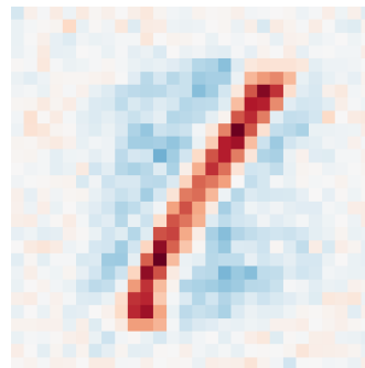
\lambda=0.10
