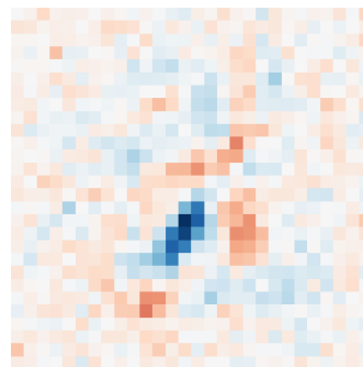
\lambda=-0.14
