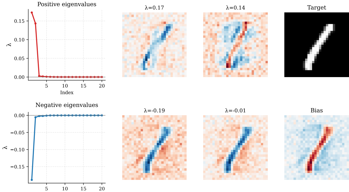
Figure 8: Challenge task eigendecomposition with full regularization (noise \sigma = 0.5 , weight decay \lambda = 1.0 ), reproducing paper Figure 6. Left: Eigenvalue decay shows dominant positive/negative modes. Middle: Top eigenvectors resemble the target digit pattern. Right: Target digit and bias visualization.
