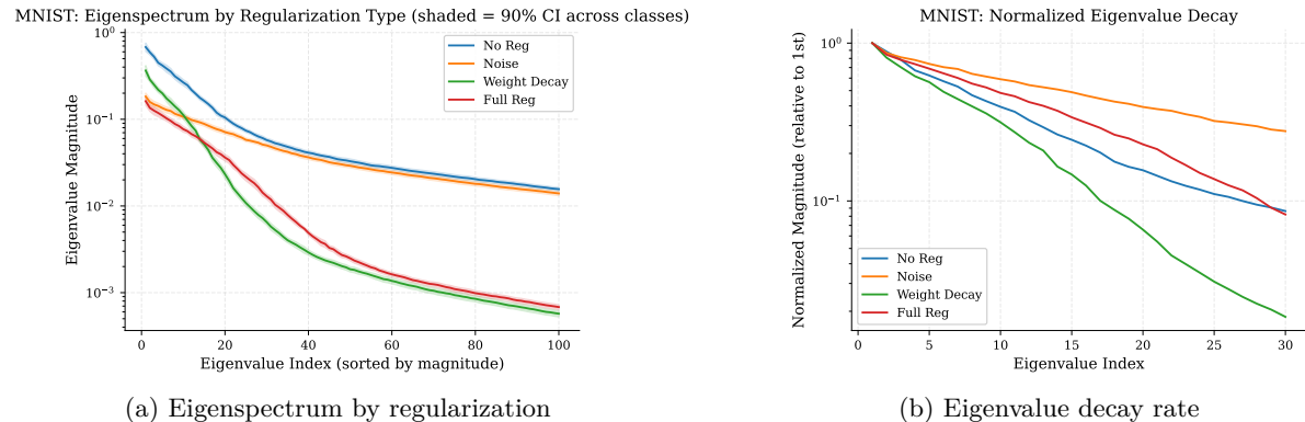
Figure 6: Eigenspectrum analysis on MNIST. Weight decay produces the steepest spectral decay, concentrating variance in 10–20 eigenvectors.
