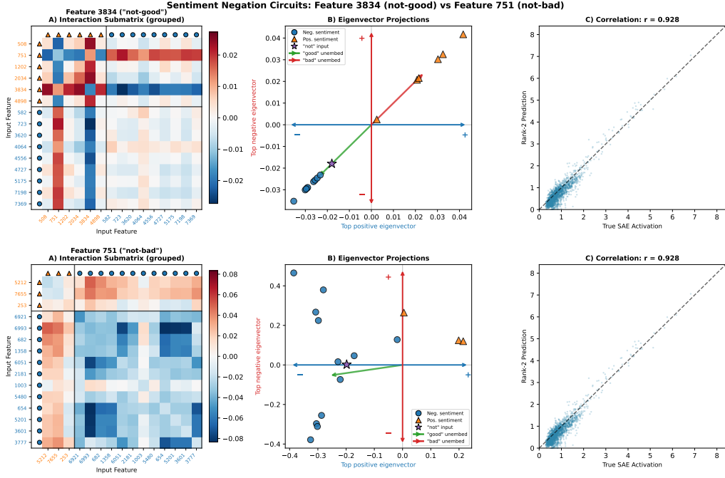
Figure 4: AND-gate circuit (fw-medium, layer 7). Top: feature 3834; bottom: feature 751. (A) Interaction submatrix, (B) eigenvector projections, (C) rank-2 vs. true activations.
