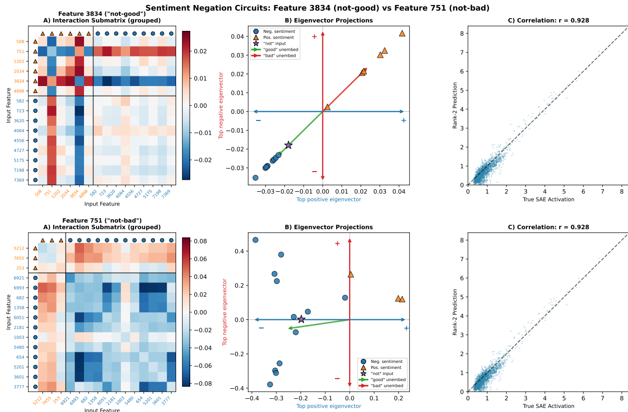
Figure 16: AND-gate circuit comparison. Top: Feature 3834 (tutorial) shows diffuse interaction structure. Bottom: Feature 751 shows clear block structure when features are grouped by cluster (black lines). The eigenvector projections (middle) separate clusters along opposite axes due to opposing eigenvalues. Scatter plots (right) show rank-2 approximation quality ( r = 0.93 , old).
