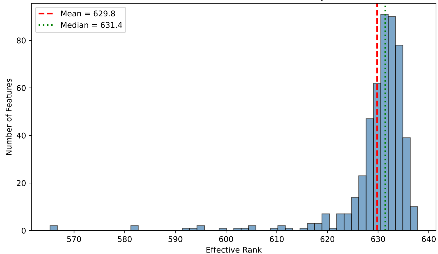
Effective Rank Distribution (fw-medium, Layer 7)
