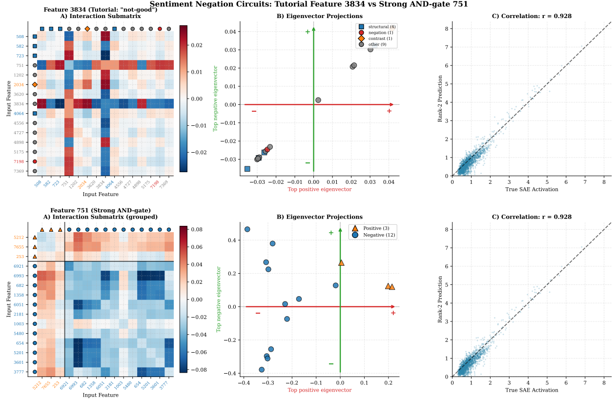
Figure 16: AND-gate circuit comparison. Top : Feature 3834 (tutorial) shows diffuse interaction structure. Bottom : Feature 751 shows clear block structure when features are grouped by cluster (black lines). The eigenvector projections (middle) separate clusters along opposite axes due to opposing eigenvalues. Scatter plots (right) show rank-2 approximation quality ( r = 0.93 ).
