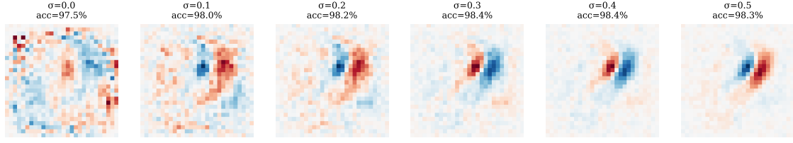
Figure 4: Top eigenvector for digit 5 across noise levels ( \sigma = 0.0 to 0.5 ). Accuracy improves with noise despite spreading variance across more eigenvectors.
