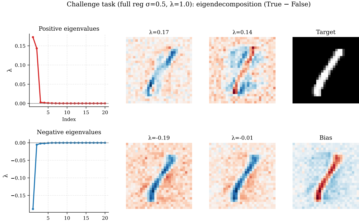
Figure 5: Challenge task eigendecomposition with full regularization (noise \sigma = 0.5 , weight decay = 1.0), reproducing paper Figure 6. Left: Eigenvalue decay shows dominant positive/negative modes. Middle: Top eigenvectors resemble the target digit pattern. Right: Target digit and bias visualization.
