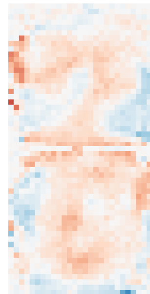
Class 7
