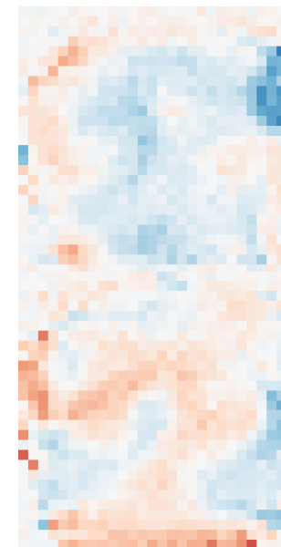
Class 8
