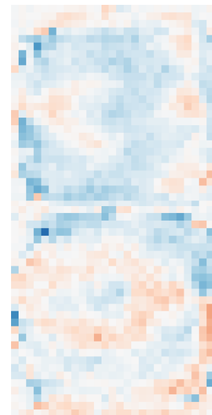
Class 3
