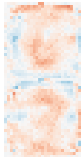
Class 6
