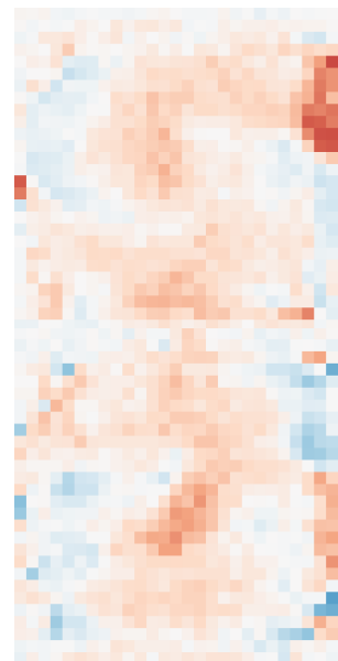
Class 5
