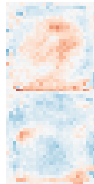
Class 9
