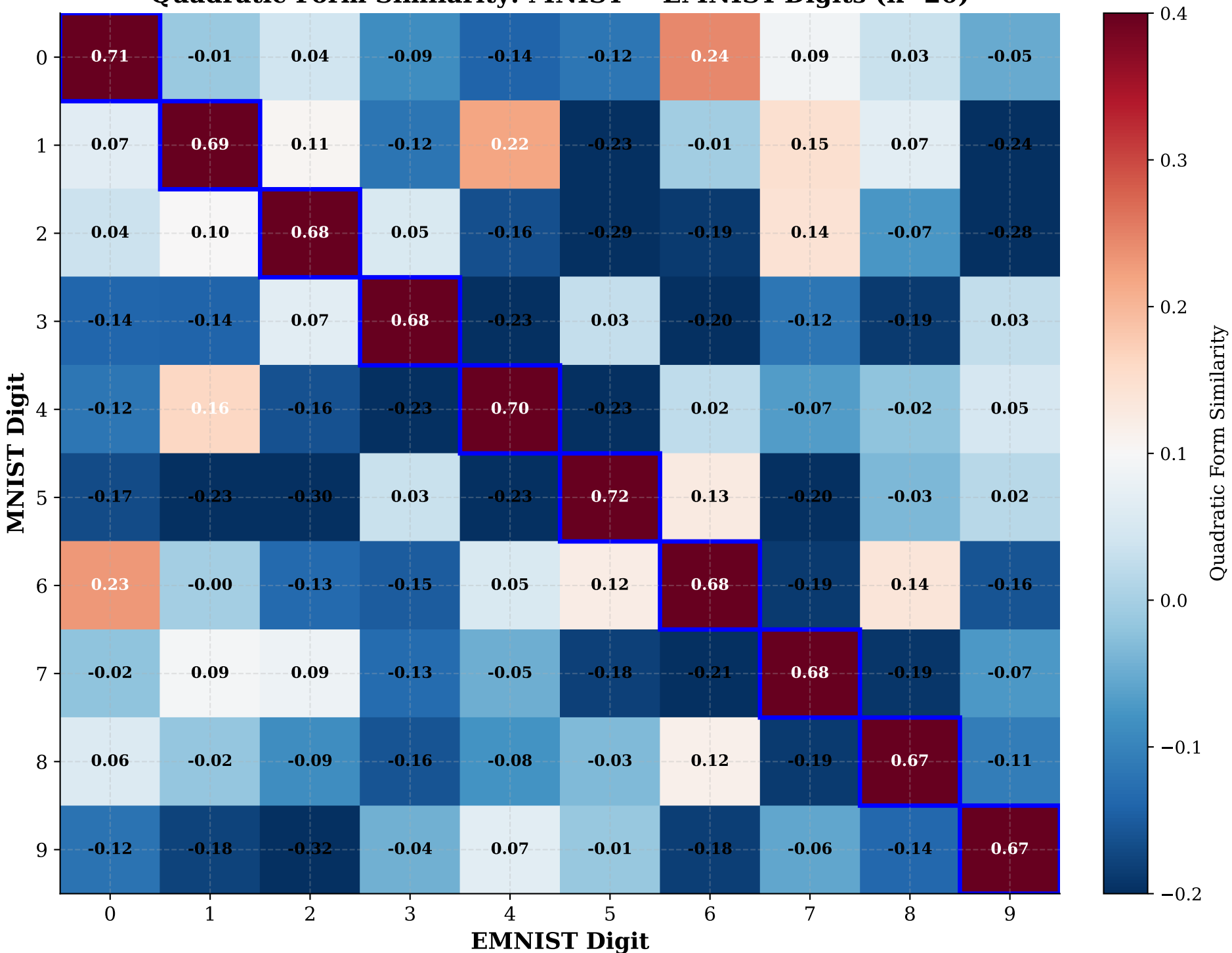
Quadratic Form Similarity: MNIST \leftrightarrow EMNIST-Digits (k=20)
