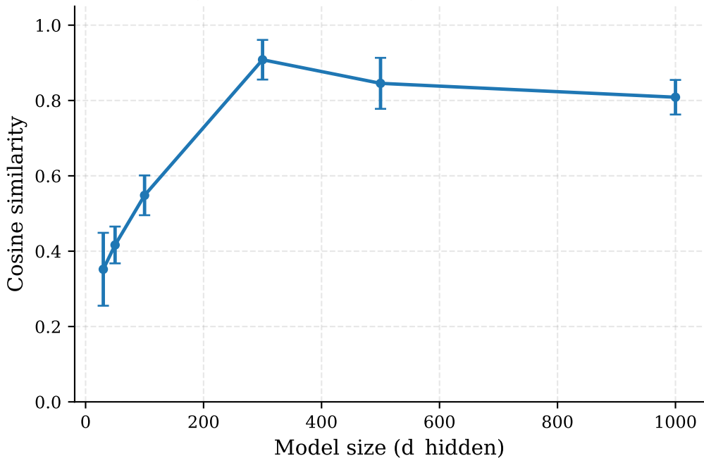
Inter-size eigenvector similarity (ref=300, top-1 per class)
