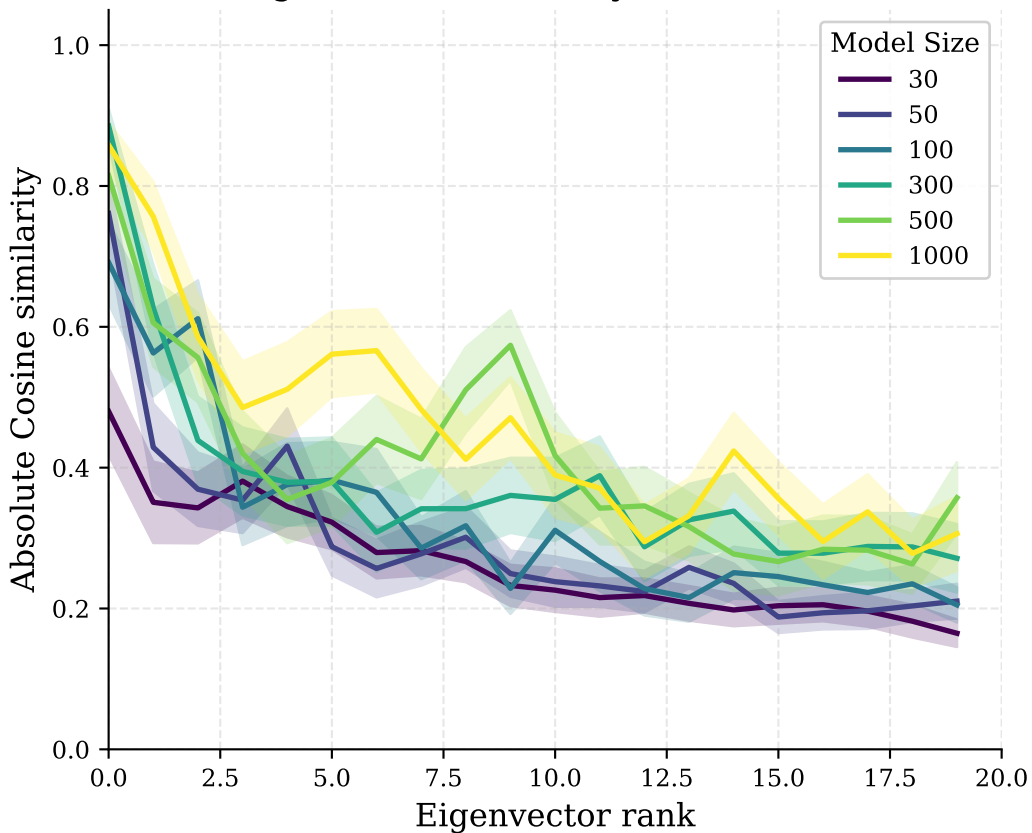
Eigenvector Similarity Across Seeds
