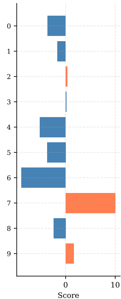
Class Scores
