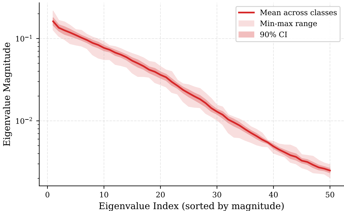
MNIST (Full Reg): Eigenspectrum Across Digit Classes
