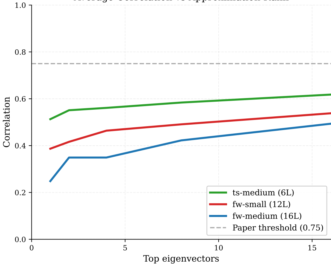
Average Correlation vs Approximation Rank
