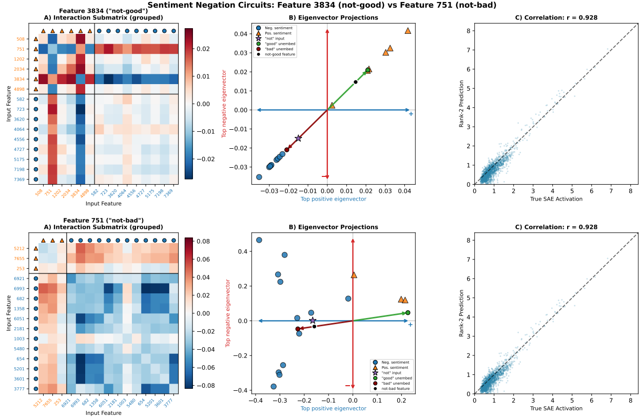
Figure 16: AND-gate circuit comparison. Top: Feature 3834 (tutorial) shows diffuse interaction structure. Bottom: Feature 751 shows clear block structure when features are grouped by cluster (black lines). The eigenvector projections (middle) separate clusters along opposite axes due to opposing eigenvalues. Scatter plots (right) show rank-2 approximation quality ( r = 0.93 , old).
