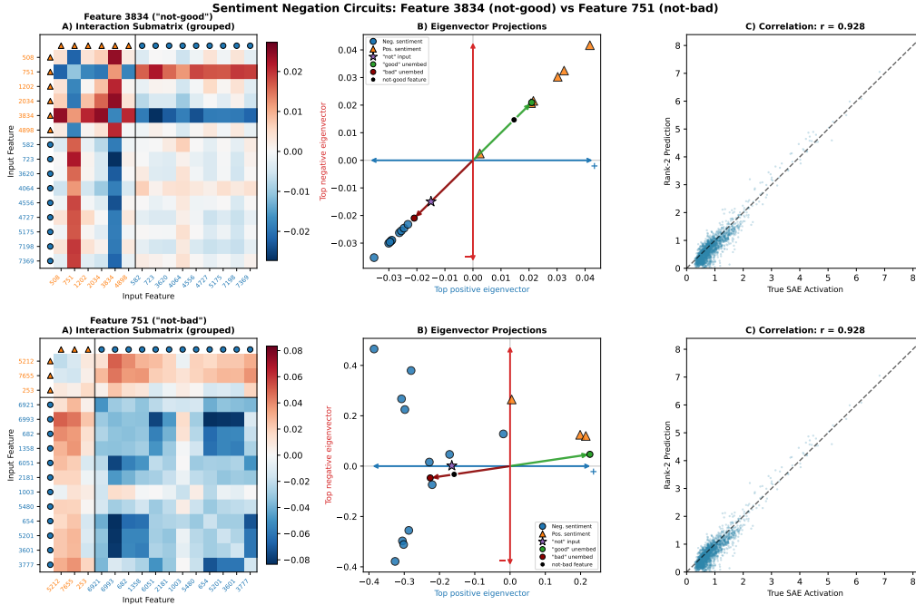
Figure 4: Negation circuit discovery ( fw-medium , layer 7). Top: feature 3834 (“not-good”); bottom: feature 751 (“not-bad”). (A) Interaction submatrix Q_f shows block structure—positive/negative sentiment features interact oppositely. (B) Eigenvector projections reveal clustering: sentiment features separate along the “good” \leftrightarrow “bad” axis.
