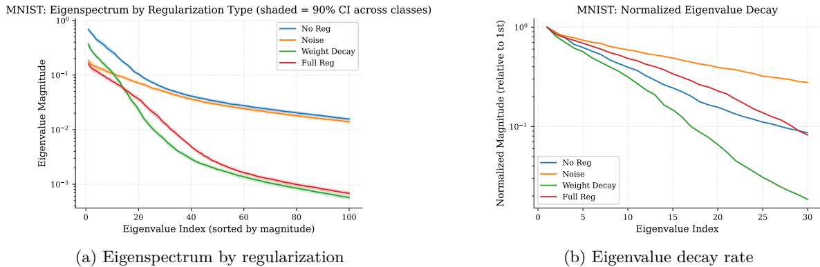
Figure 2: Eigenspectrum analysis on MNIST. Weight decay produces the steepest spectral decay, concentrating variance in 10–20 eigenvectors.
