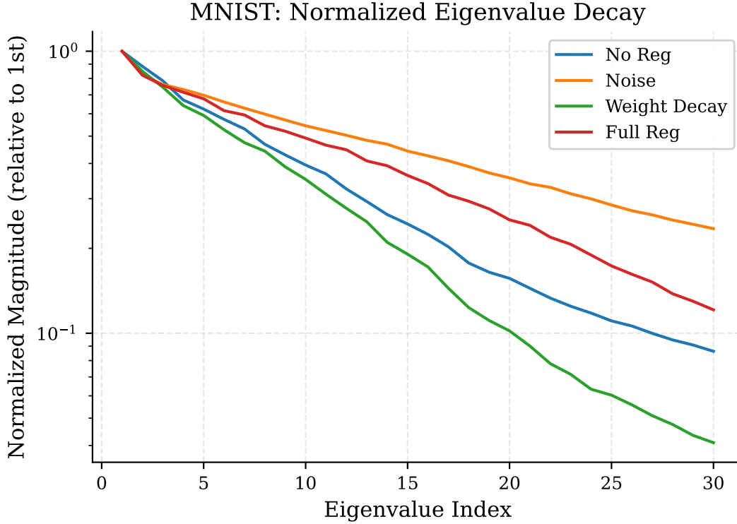
Figure 2: Normalized eigenvalue decay for top-30 eigenvalues. Values are normalized by the maximum eigenvalue per configuration. Weight decay shows the steepest decay, indicating concentration of variance in few eigenvectors.
