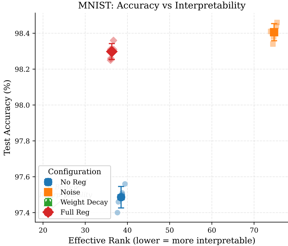
Figure 6: Accuracy vs effective rank trade-off on MNIST. Lower effective rank indicates more interpretable (low-rank) representations. Each point represents one seed; colors indicate configuration.
