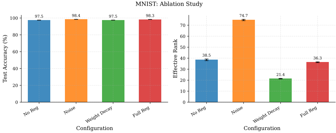
Figure 5: Ablation study visualization for MNIST showing accuracy and effective rank across regularization configurations. Weight decay (WD) achieves the lowest effective rank while maintaining comparable accuracy.
