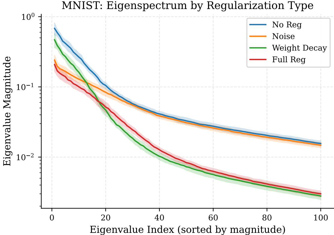
Figure 1: Eigenspectrum comparison across regularization configurations on MNIST. Weight decay (WD) produces the sharpest spectral decay, while noise augmentation alone increases effective rank. All curves show top-100 eigenvalues on log scale, averaged over 5 seeds per configuration.
