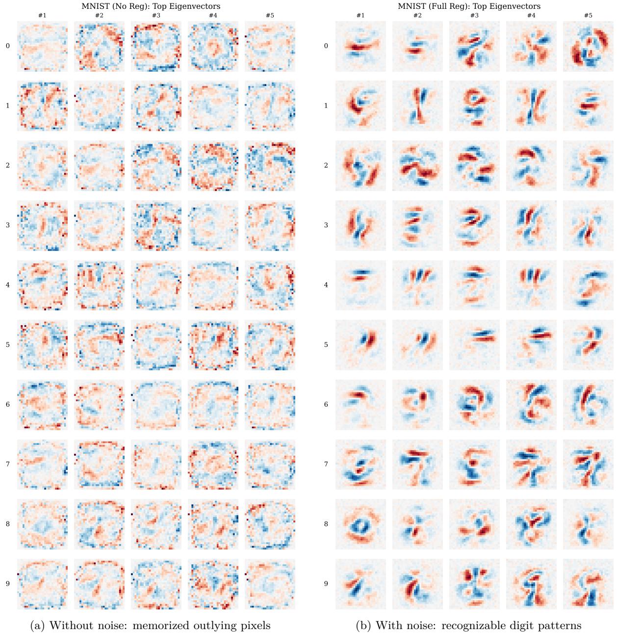
Figure 4: Top-5 eigenvectors (by eigenvalue magnitude) for each digit class (0–9). Without noise augmentation, the model memorizes specific outlying pixel patterns that rarely occur, resulting in diffuse, uninterpretable eigenvectors. With noise augmentation, the model learns generalizable features, producing eigenvectors that resemble recognizable digit strokes. Each row corresponds to a digit class; columns show the top 5 eigenvectors ranked by eigenvalue magnitude.
