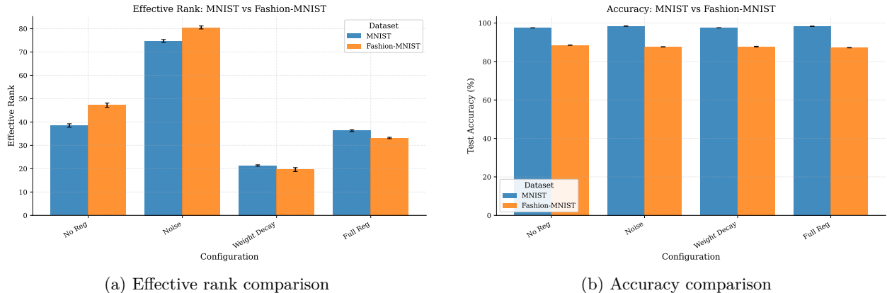
Figure 7: Cross-dataset comparison between MNIST and Fashion-MNIST. Both datasets show consistent trends across regularization configurations.
