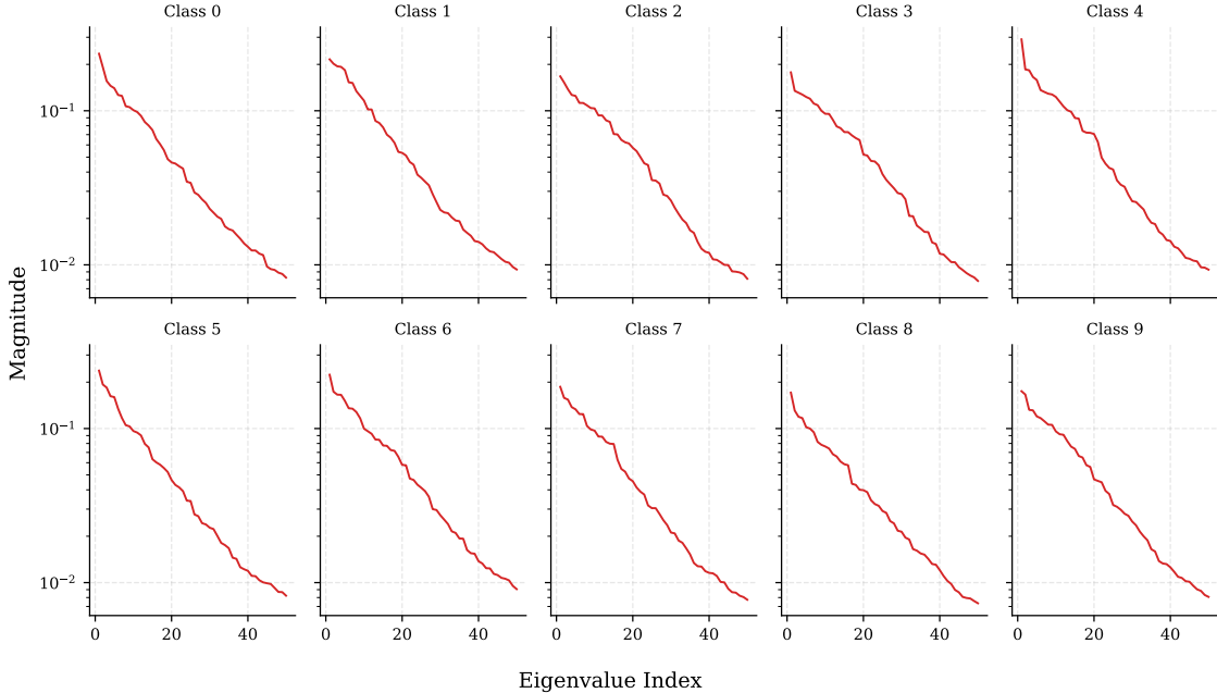
Figure 3: Per-class eigenspectrum for the fully regularized MNIST model. Each line represents a digit class (0–9). All classes show similar low-rank structure, consistent with the paper’s claims about class-specific interpretability.
