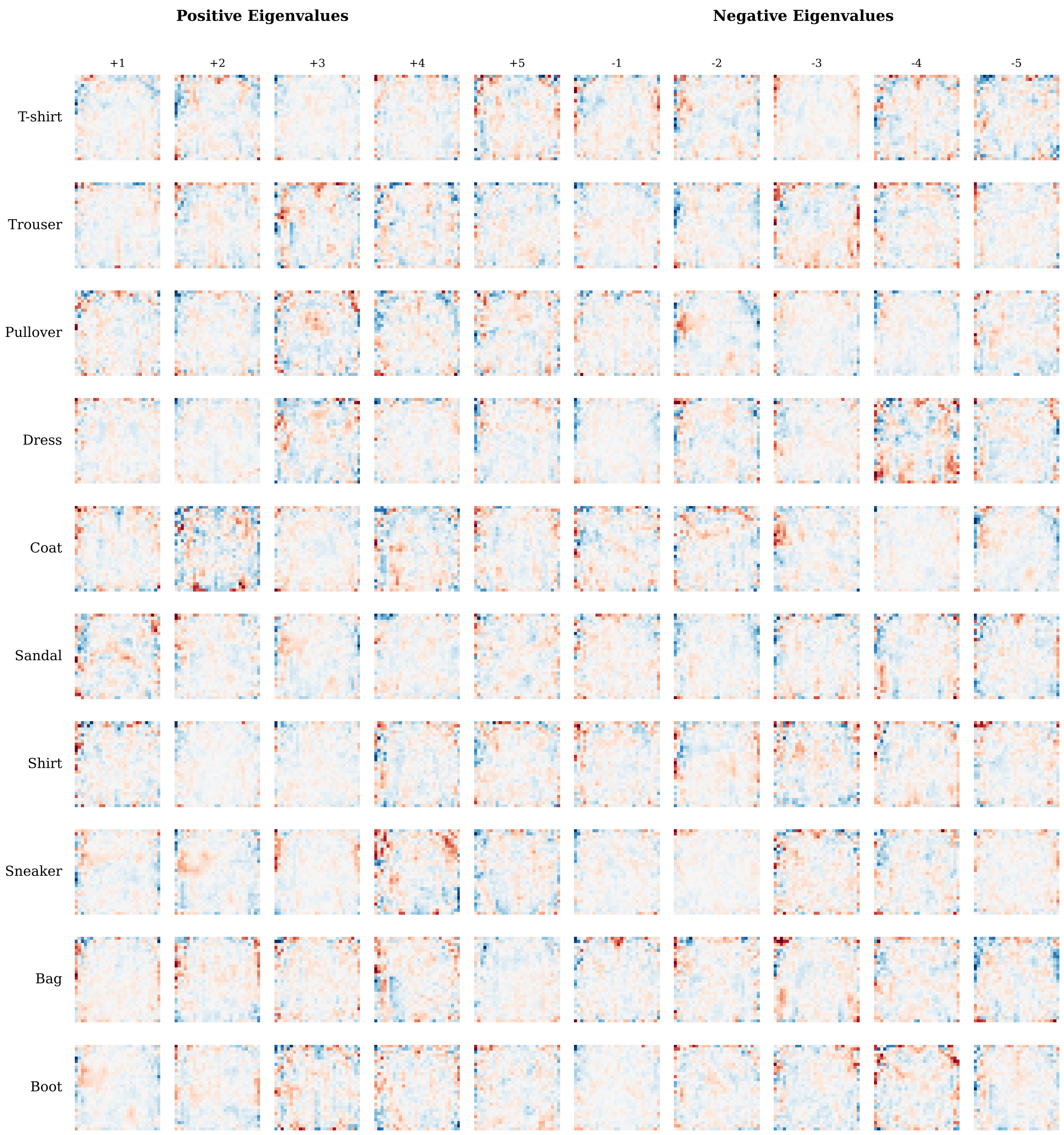
Fashion-MNIST (No Reg): Top Eigenvectors
