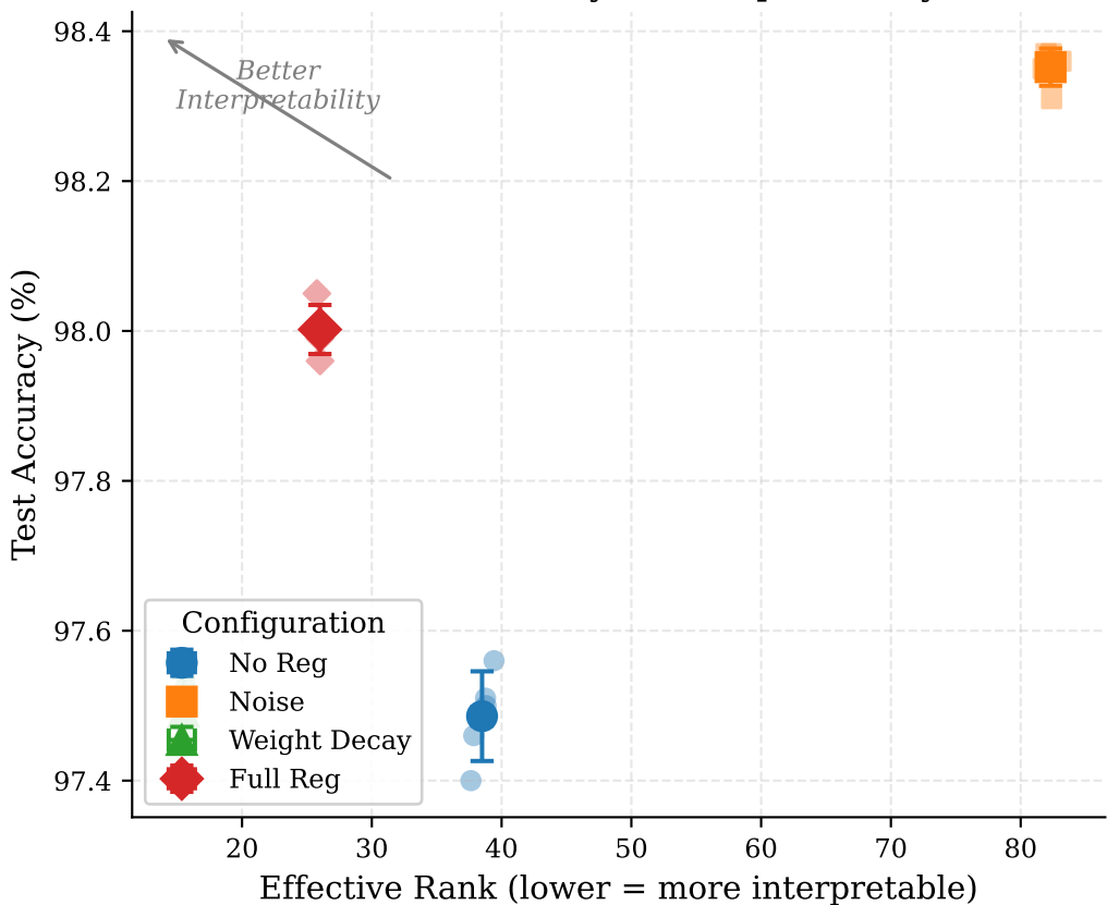
MNIST: Accuracy vs Interpretability
