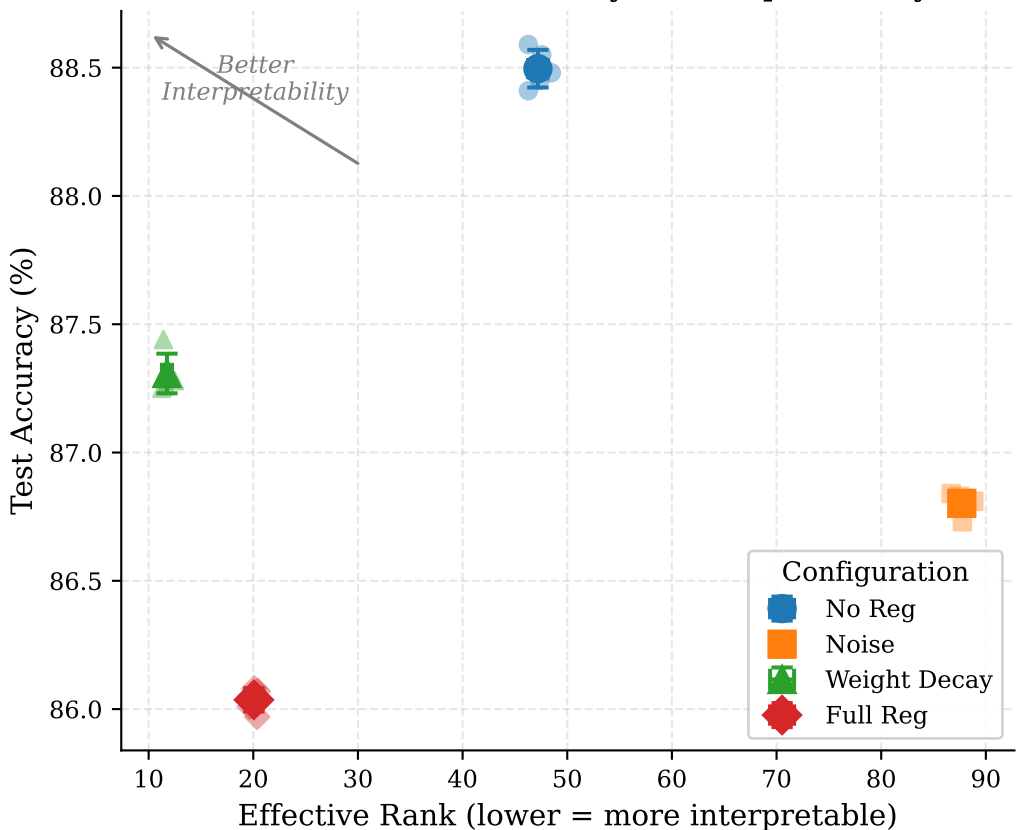
Fashion-MNIST: Accuracy vs Interpretability
