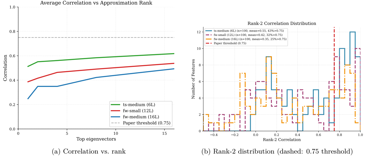
Figure 4: Low-rank correlation analysis (Paper Figure 9). Mean correlation improves with rank but remains below paper’s reported values. The 0.75 threshold is achieved by fewer features than claimed.
