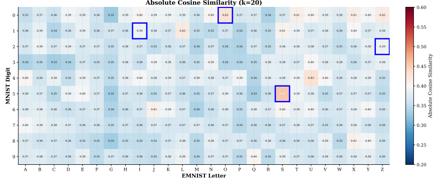
Figure 13: Absolute cosine similarity between MNIST digit classes and EMNIST letter classes fails to distinguish geometrically similar pairs (0-O) from dissimilar pairs (0-X).
