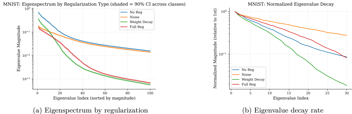
Figure 2: Eigenspectrum analysis on MNIST. Weight decay produces the steepest spectral decay, concentrating variance in 10–20 eigenvectors.
