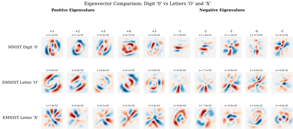
Figure 10: Three-way eigenvector comparison: MNIST-0, EMNIST-O, and EMNIST-X. The top eigenvectors for each class are visually distinct from one another
