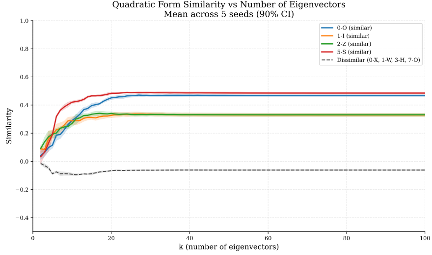
Figure 7: Quadratic Form Similarity vs number of eigenvectors k . Similar pairs converge around k = 20 ; dissimilar pairs stay near zero with non-overlapping 90% CIs.
