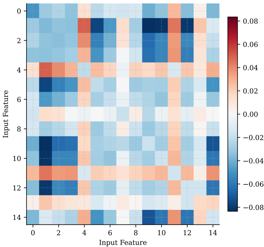
Feature 751 (Best) Interaction Submatrix
