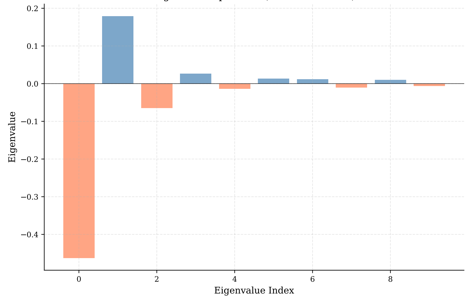
Eigenvalue Spectrum (AND-score: 0.96)
