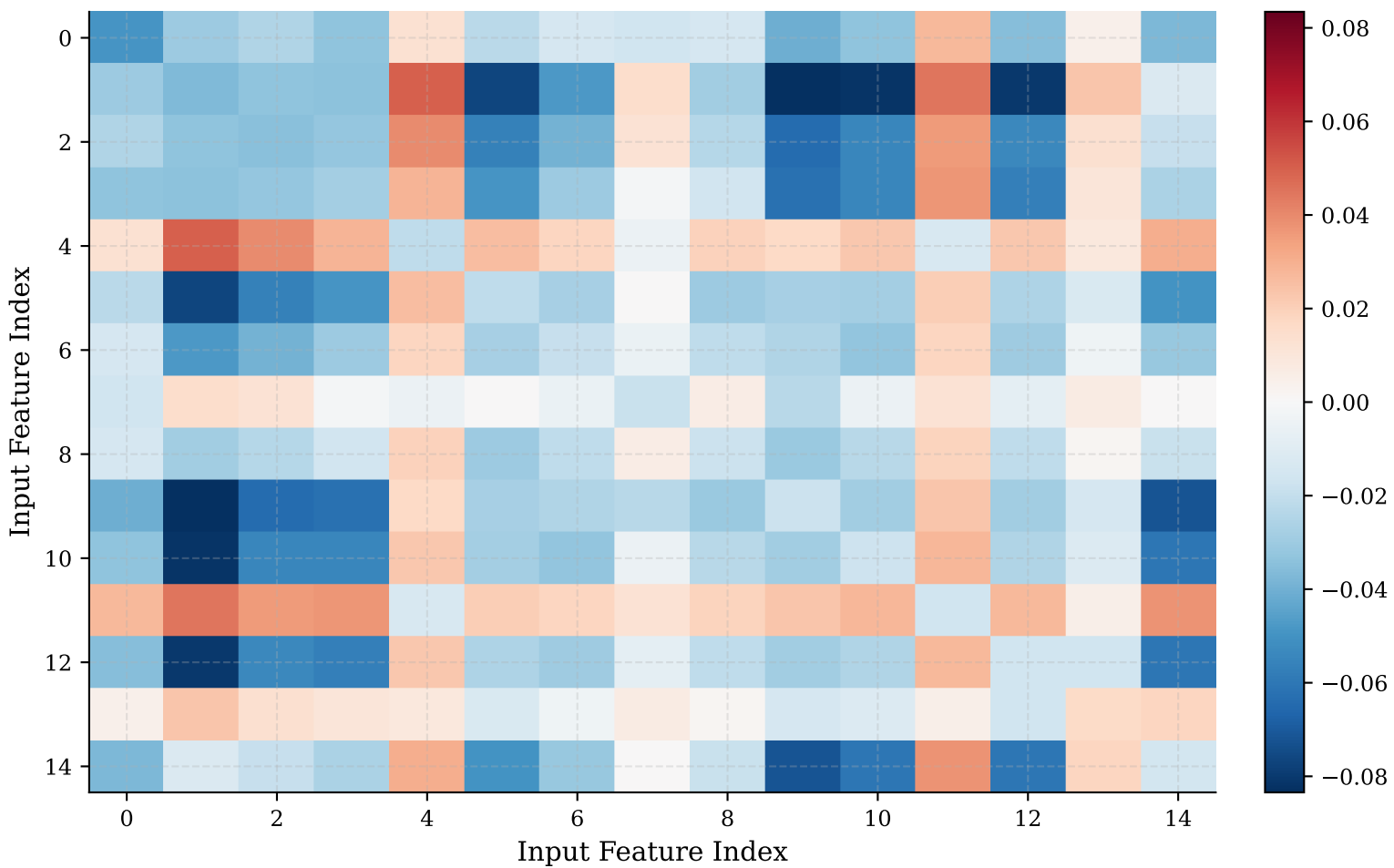
Feature 751: Interaction Submatrix
