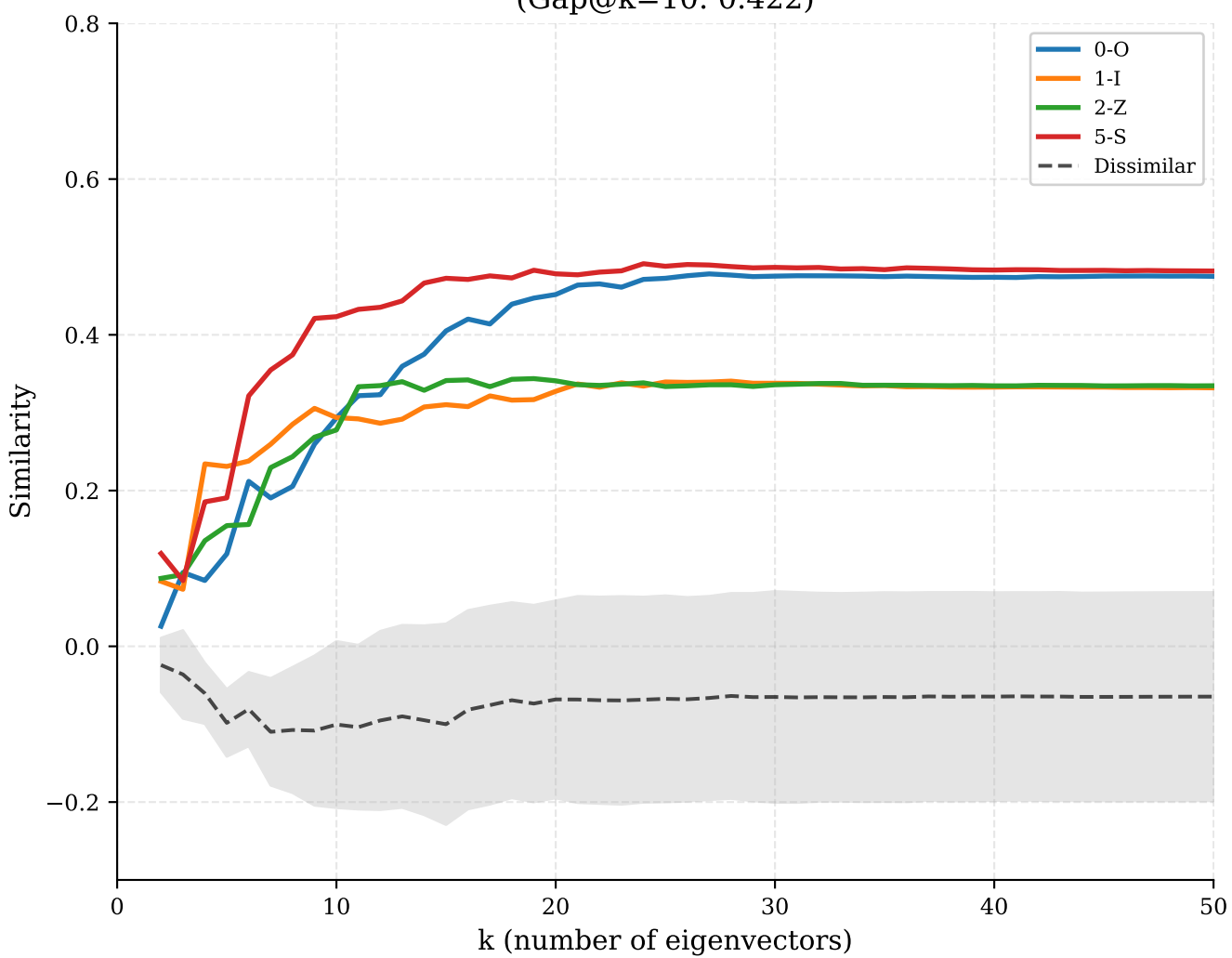
Quadratic Form (Gap@k=10: 0.422)
