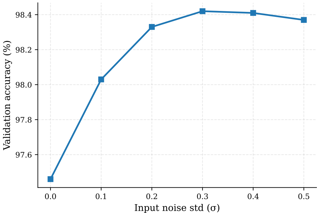
Effect of input noise on accuracy
