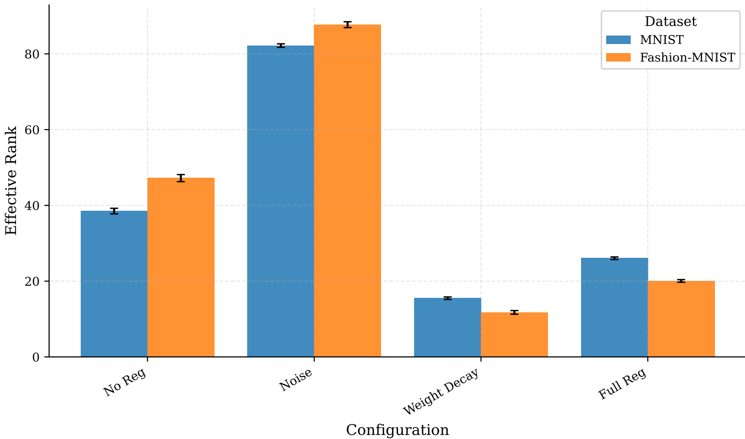
Effective Rank: MNIST vs Fashion-MNIST
