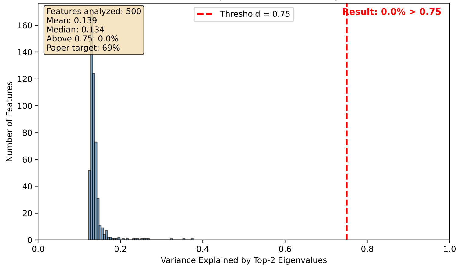
Rank-2 Variance Explained (fw-medium, Layer 7)
