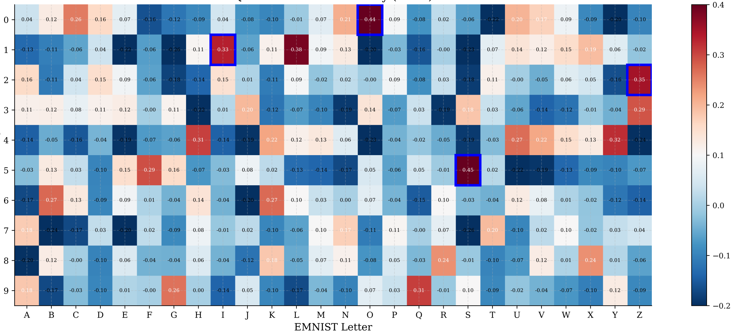
Quadratic Form Similarity (k=20)
