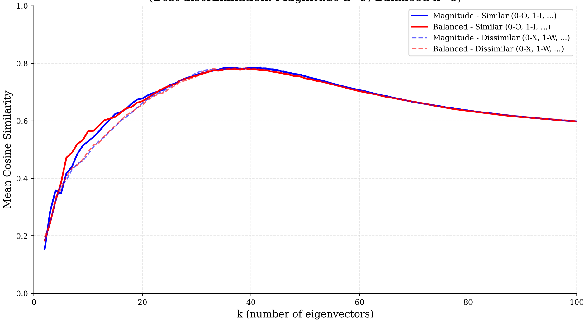
Selection Method Comparison (Best discrimination: Magnitude k=9, Balanced k=8)
