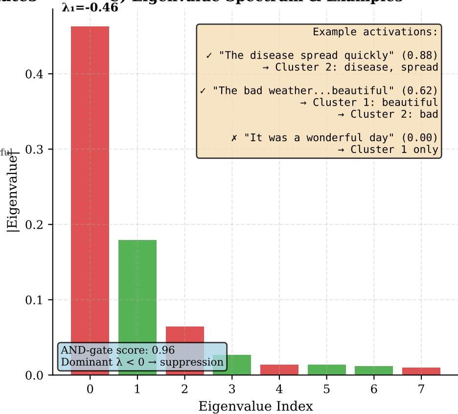
C) Eigenvalue Spectrum & Examples
