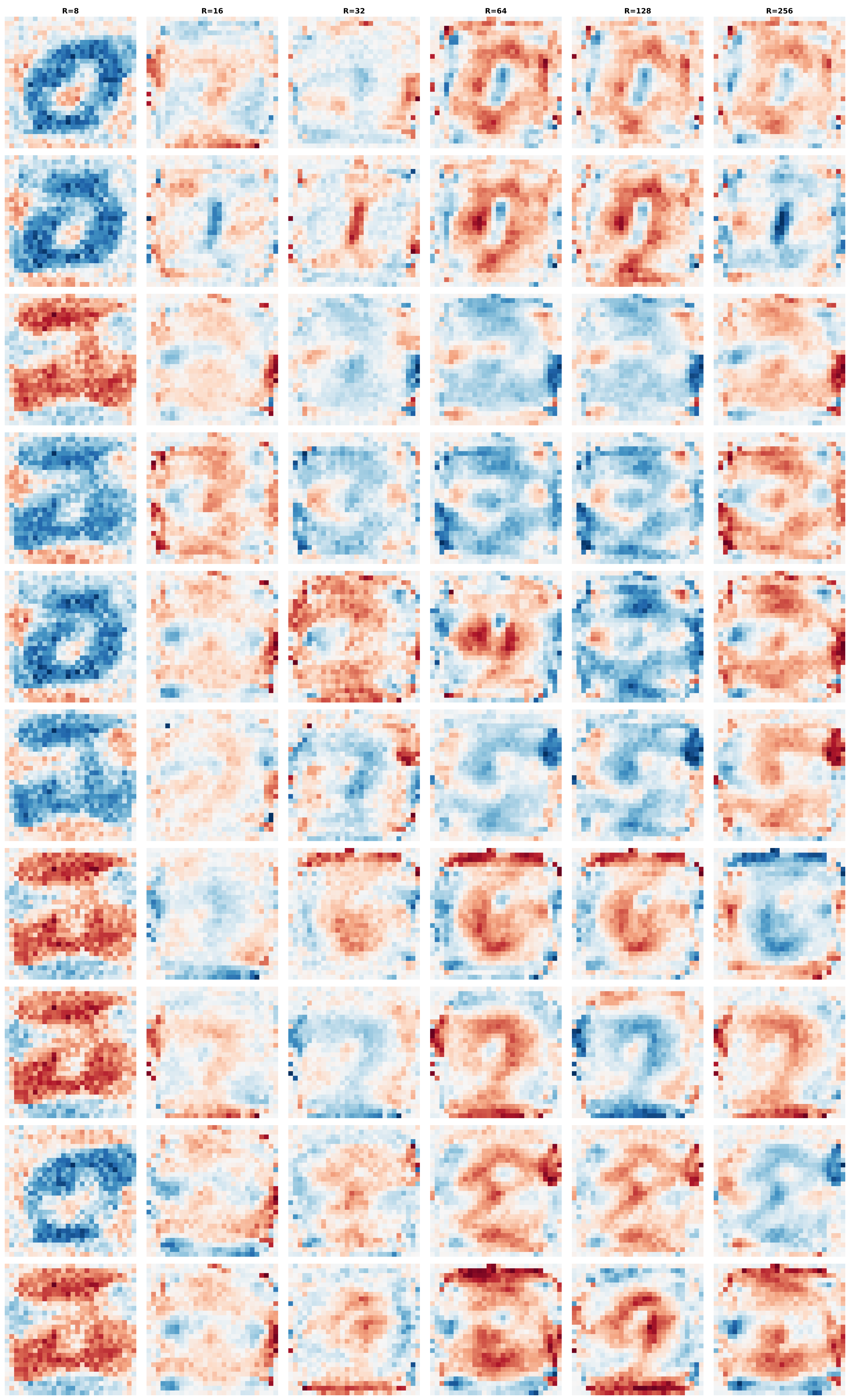
Top Eigenvector per Class Across CP Ranks
