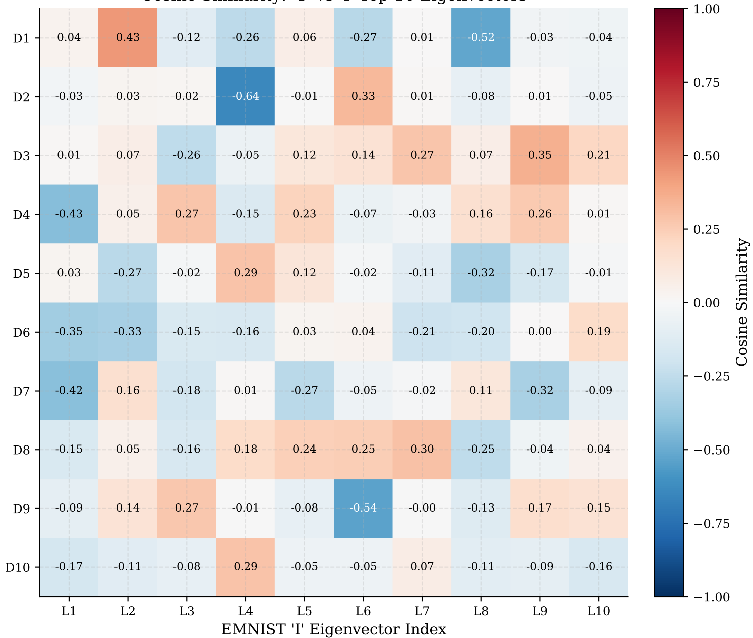
Cosine Similarity: 'l' vs 'I' Top-10 Eigenvectors
