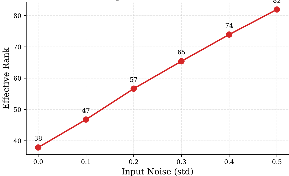
Effect of Input Noise on Effective Rank
