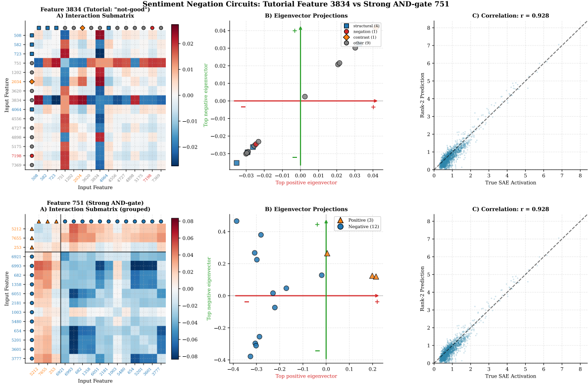
Figure 13: AND-gate circuit comparison (fw-medium, layer 7). Top: Feature 3834 (tutorial) shows diffuse structure (old). Bottom: Feature 751 (AND-score 0.96, old) shows clear block structure with opposing eigenvalues ( \lambda_1 < 0 , \lambda_2 > 0 ) (old). Axes in (B) show projection onto top eigenvectors; clusters separate along these directions. Updated plot pending rerun.
