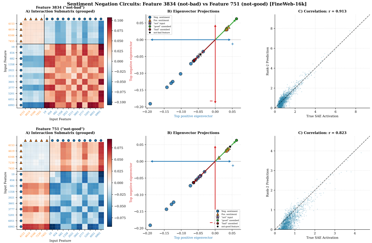
Figure 16: AND-gate circuit on FineWeb-16k (model’s training distribution). Correlations: 0.91 (feature 3834), 0.82 (feature 751). Feature 751 activates more frequently on FineWeb-16k (6,517 vs 2,542 samples), likely due to more “not-good” contexts in educational/scientific text.
