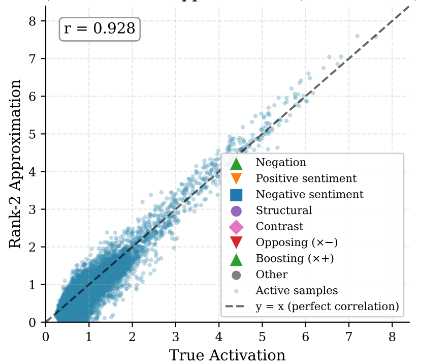
C) Activation vs Approximation (Feature 3834)
